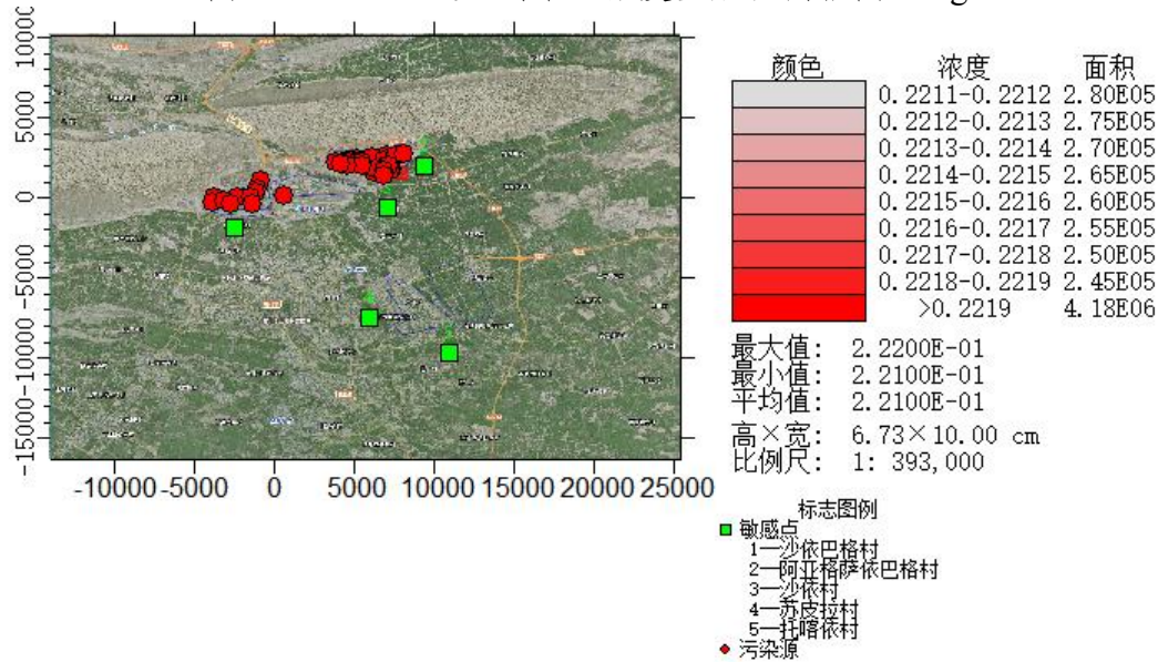
图5-2-13 \text{PM}_{10} 日均落地浓度叠加值网格图 ( \text{mg}/\text{m}^3 )
